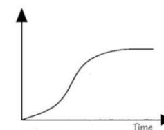
S-Shaped Growth
